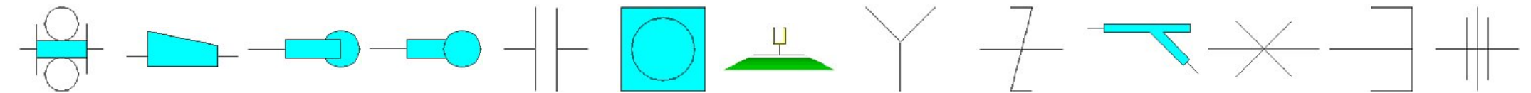
Double basket strainer Eccentric reducer Elbow facing down Elbow facing up Flanged pipe joint Floor drain Football goalpost Funnel drain Grooved mechanical joint Lateral Pipe anchor Pipe cap Pipe union
