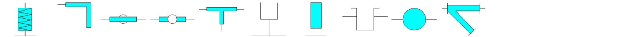
Spring hanger Square elbow Tee down Tee up Tee Temperature and pressure tap Thermometer in a well Thermometer well Welded pipe joint Y-type strainer
