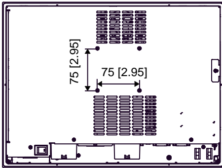
PS-3710A Rear (PS3710A-T41)
