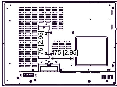
PS-3711A Rear (PS3711A-T41-24V)
