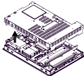
PS3711A-T41-24V
