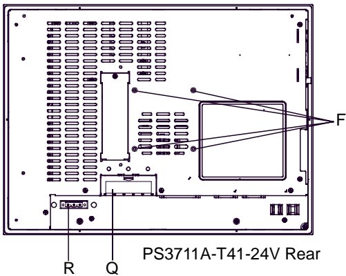
PS3711A-T41 Rear
